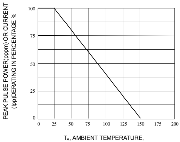
Fig. 2-PULSE DERATING CURVE
