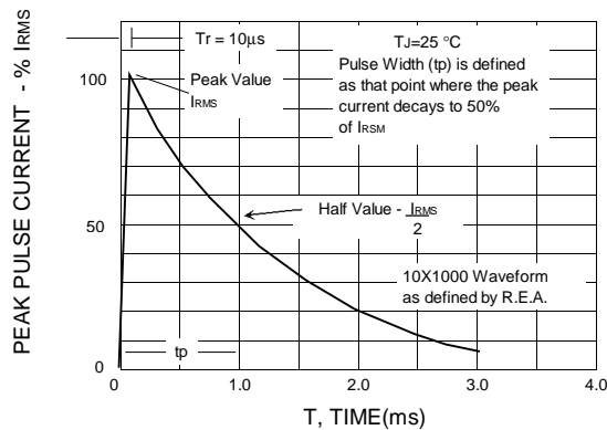
FIG.5 - PULSE WAVEFORM
