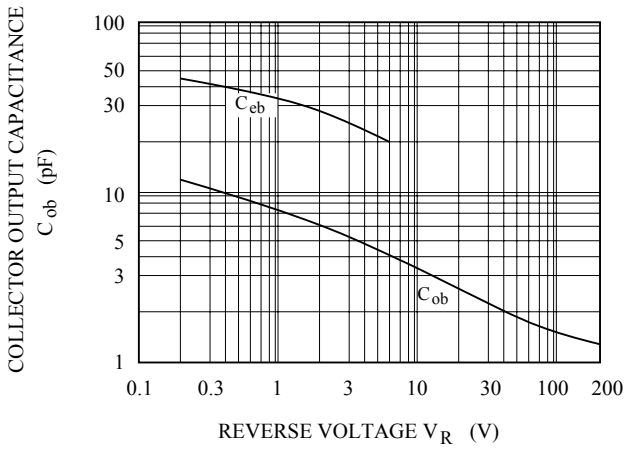
C_{ob} - V_R
