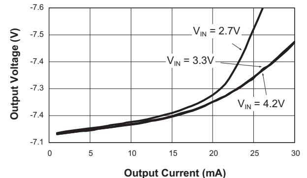
Negative Charge Pump Output vs. Output Current (No Load at V_{POS} and V_{OUT} )
