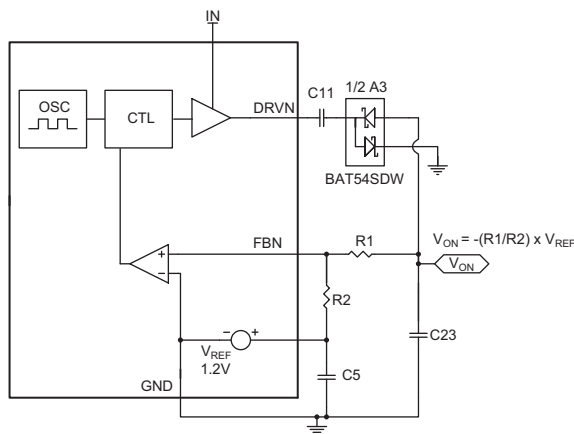
Figure 1: Negative Charge Pump Block Diagram.
