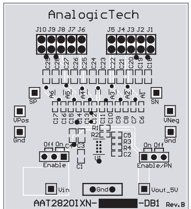
Figure 5: AAT2820 Evaluation Board Bottom Side Layout.
