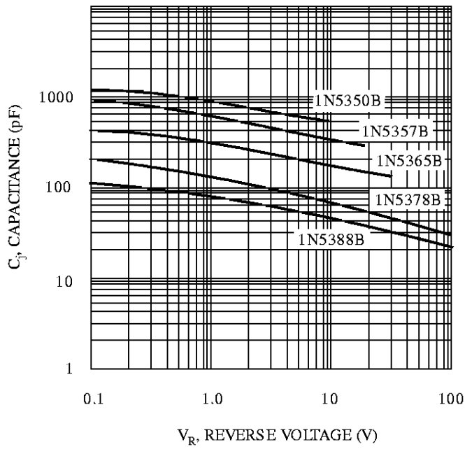
Fig. 1, Typ. Capacitance vs. Reverse Voltage
