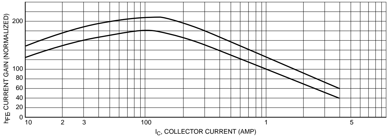
Figure 2. Current Gain
