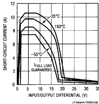
LT1083 Short-Circuit Current
