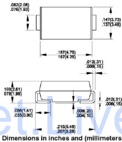
DO-214AA (SMB)
