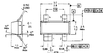
SOT-143 TOP VIEW
