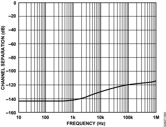
Figure 50. Channel Separation vs. Frequency
