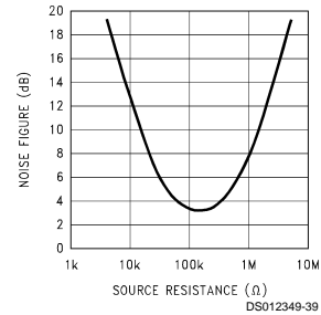
NF vs Source Resistance
