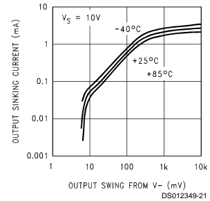
Output Voltage vs Sinking Current
