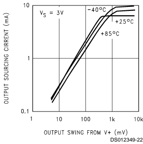
Output Voltage vs Sourcing Current
