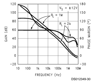
Gain and Phase vs Frequency
