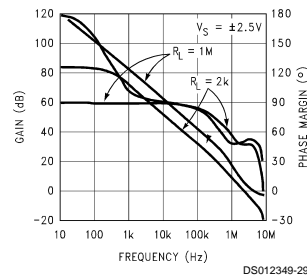
Gain and Phase vs Frequency
