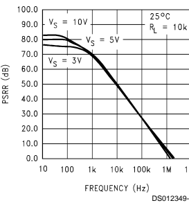
Pos PSRR vs Frequency
