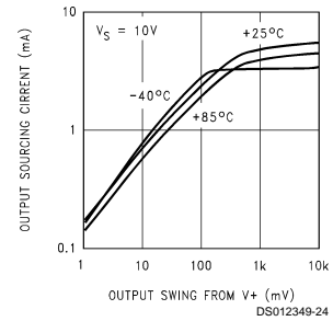
Output Voltage vs Sourcing Current
