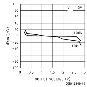
dV_{OS} vs Output Voltage
