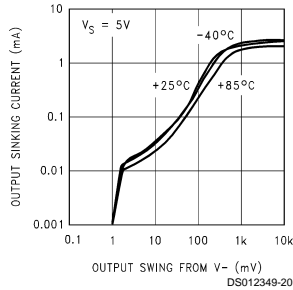
Output Voltage vs Sinking Current
