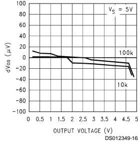
dV_{OS} vs Output Voltage
