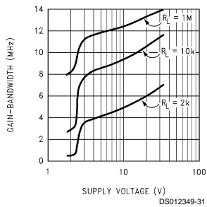
GBW vs Supply Voltage at 20 kHz
