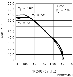
Neg PSRR vs Frequency
