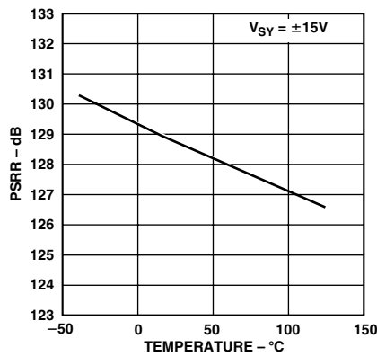
TPC 23. PSRR vs. Temperature
