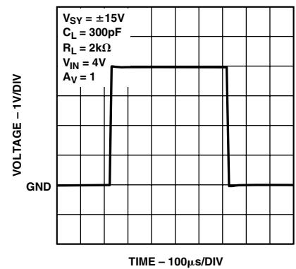
TPC 9. Large Signal Transient Response
