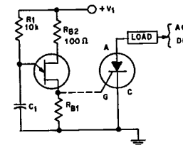
Fig. 22—Circuit for minimum supply voltage curves, Fig. 21.
