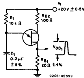
Fig. 2—Typical base-1 peak-pulse voltage circuit.
