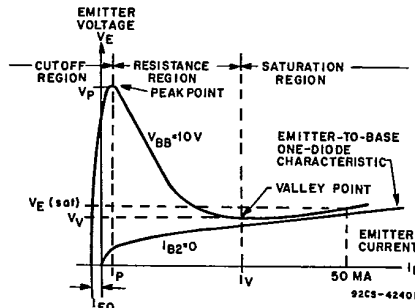
Fig. 3—Static emitter characteristics waveforms.
