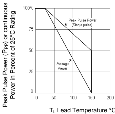
FIGURE 3 Derating Curve
