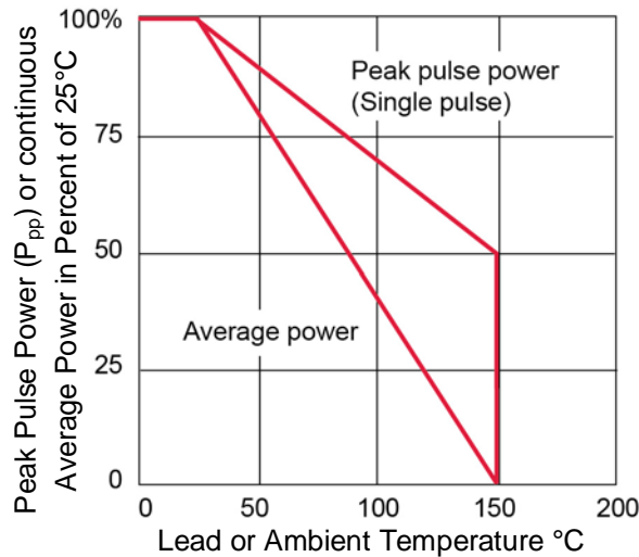
FIGURE 4 Derating Curve
