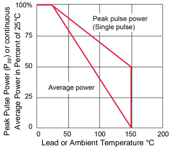
FIGURE 4 Derating Curve
