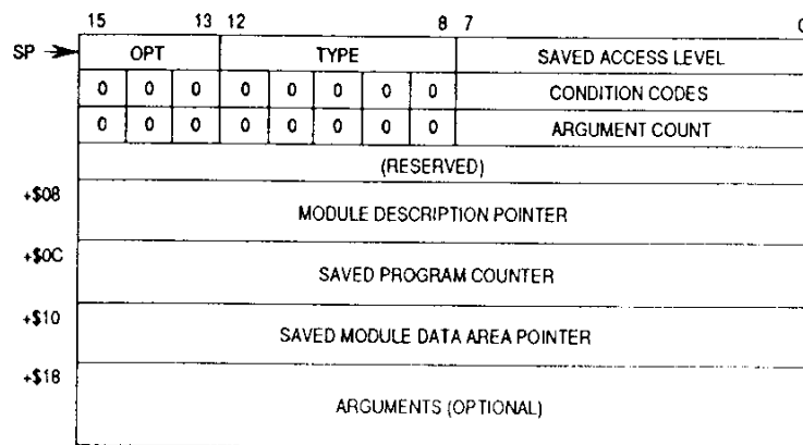
Figure 9-12. Module Call Stack Frame
