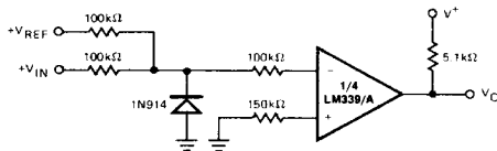
Comparing Input Voltages of Opposite Polarity
