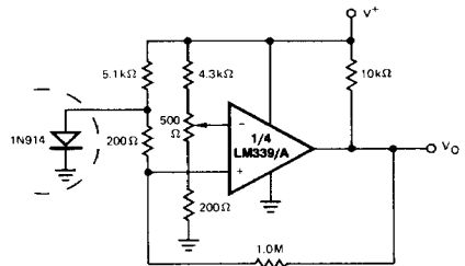
LIC-114
