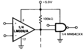
Driving CMOS
