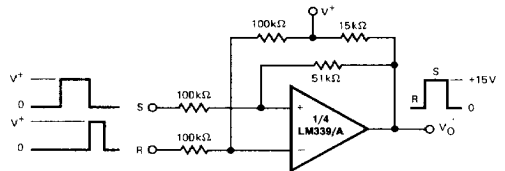
Bi-Stable Multivibrator
