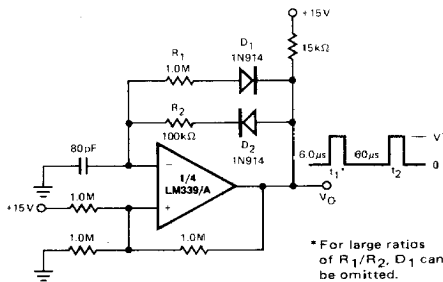
Pulse Generator
