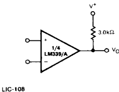
LIC-108
