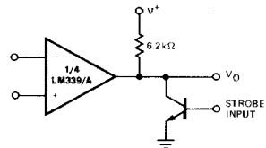
Output Strobing
