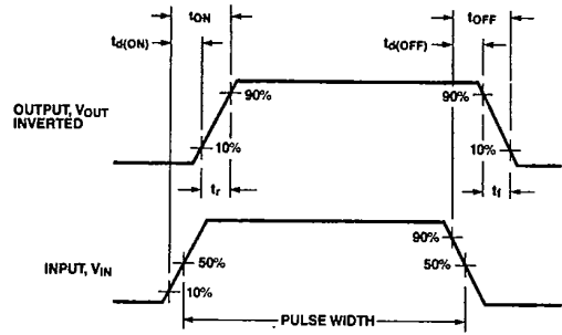
Figure 2 Switching Waveforms
