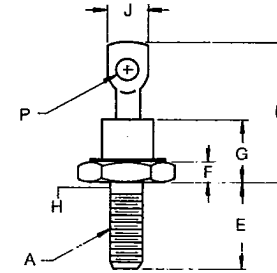
DO-203AA (DO-4)
