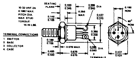
TO-111 (ISOLATED)
