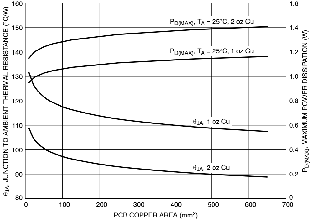
Figure 48. θ JA and P D (MAX) vs. Copper Area (CSP4)
