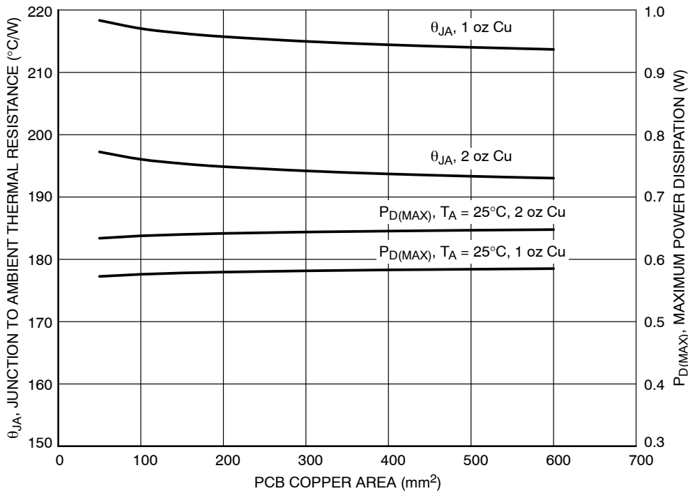
Figure 49. θ JA and P D (MAX) vs. Copper Area (XDFN4)
