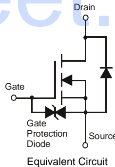
Equivalent Circuit
