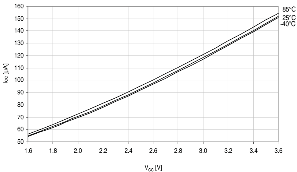
Figure 33-11. Idle mode supply current vs. V_{CC} .
