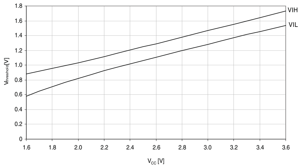
Figure 33-32. I/O pin input threshold voltage vs. V_{CC} . T = 25^{\circ}C .
