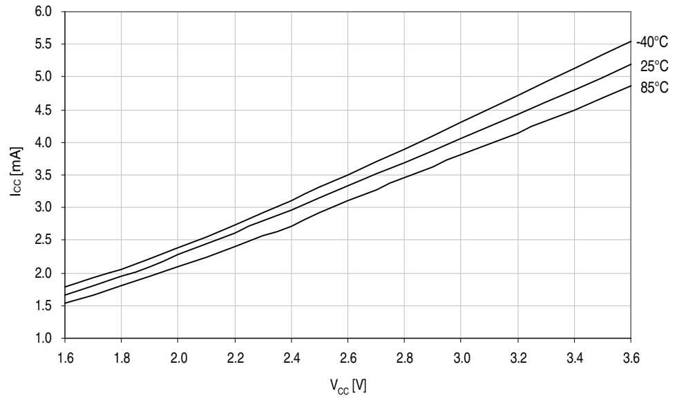
Figure 33-6. Active mode supply current vs. V_{CC} . f_{SYS} = 32MHz internal oscillator prescaled to 8MHz.
