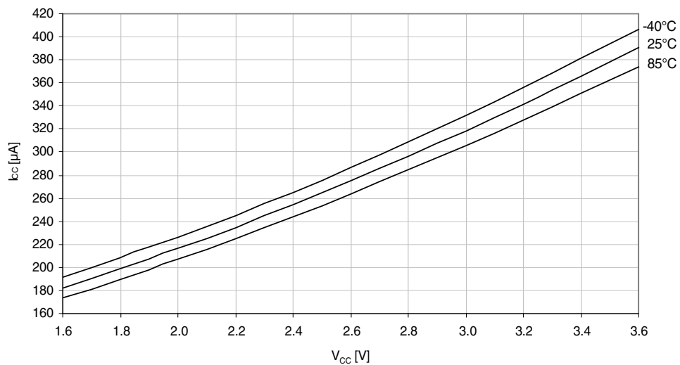
Figure 33-12. Idle mode supply current vs. V_{CC} .
