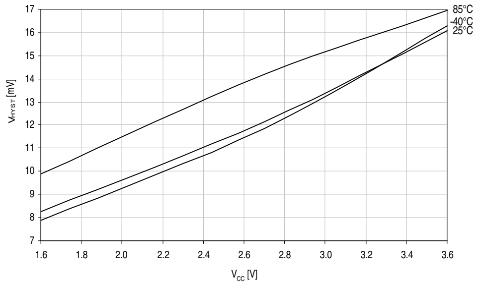
Figure 33-36. Analog comparator hysteresis vs. V_{CC} .
