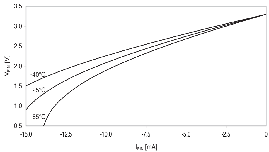
Figure 33-26. I/O pin output voltage vs. source current.
