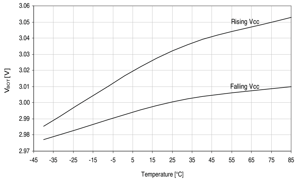
Figure 33-43. BOD thresholds vs. temperature.
