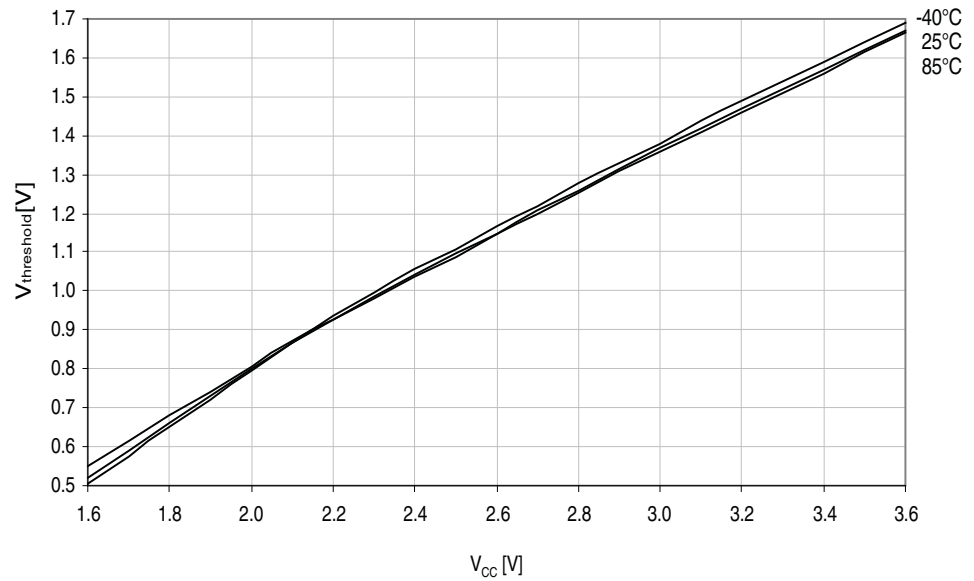
Figure 33-49. Reset pin input threshold voltage vs. V_{CC} . V_{IL} - Reset pin read as "0".
