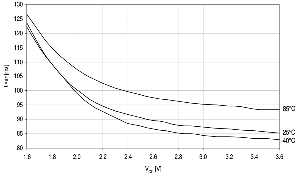
Figure 33-44. Minimum reset pin pulse width vs. V_{CC} .
