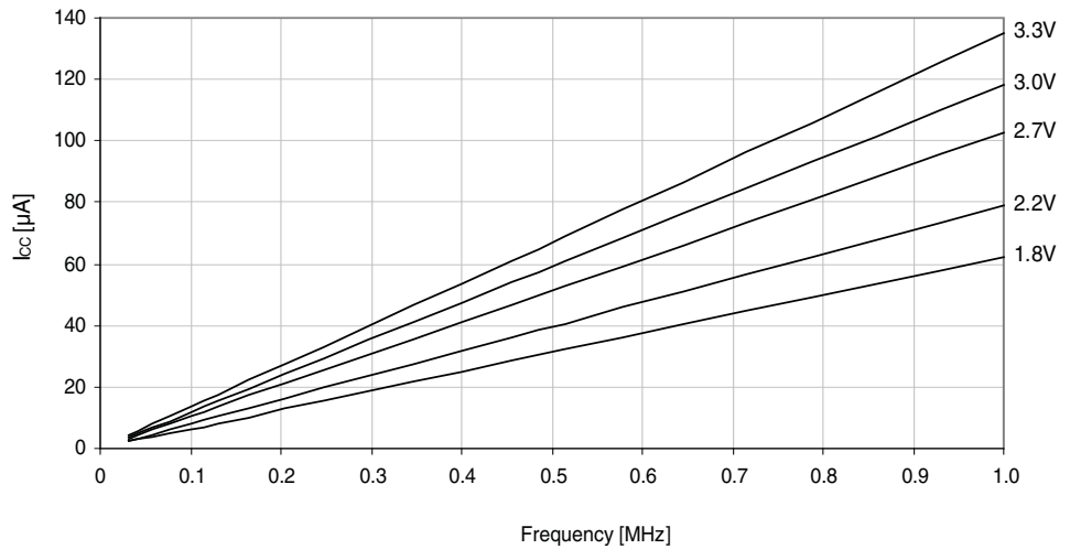
Figure 33-8. Idle mode supply current vs. frequency. f_{SYS} = 0 - 1MHz external clock, T = 25^\circ C .
