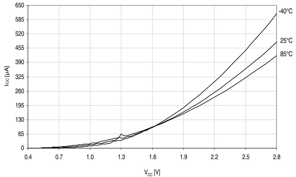
Figure 33-51. Power-on reset current consumption vs. V_{CC} . BOD level = 3.0V, enabled in sampled mode.
