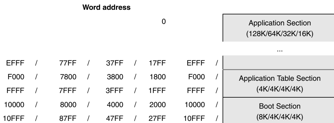
Figure 7-1. Flash program memory (Hexadecimal address).
