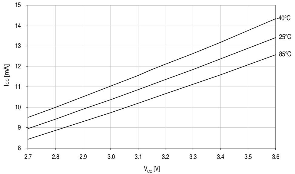
Figure 33-7. Active mode supply current vs. V_{CC} . f_{SYS} = 32MHz internal oscillator.
