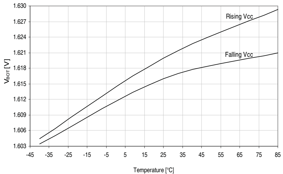
Figure 33-42. BOD thresholds vs. temperature.
