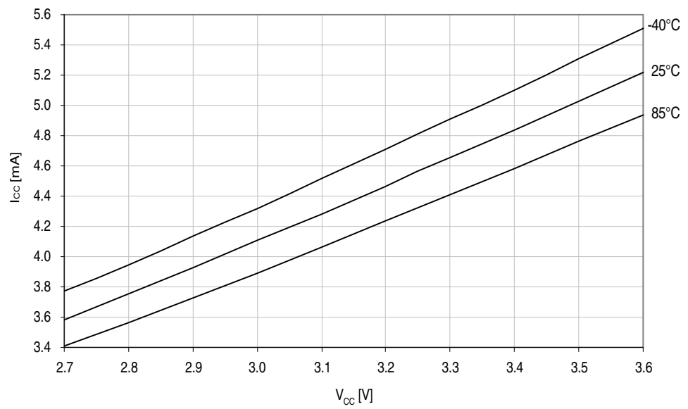
Figure 33-14. Idle mode current vs. V_{CC} . f_{SYS} = 32\text{MHz} internal oscillator.
