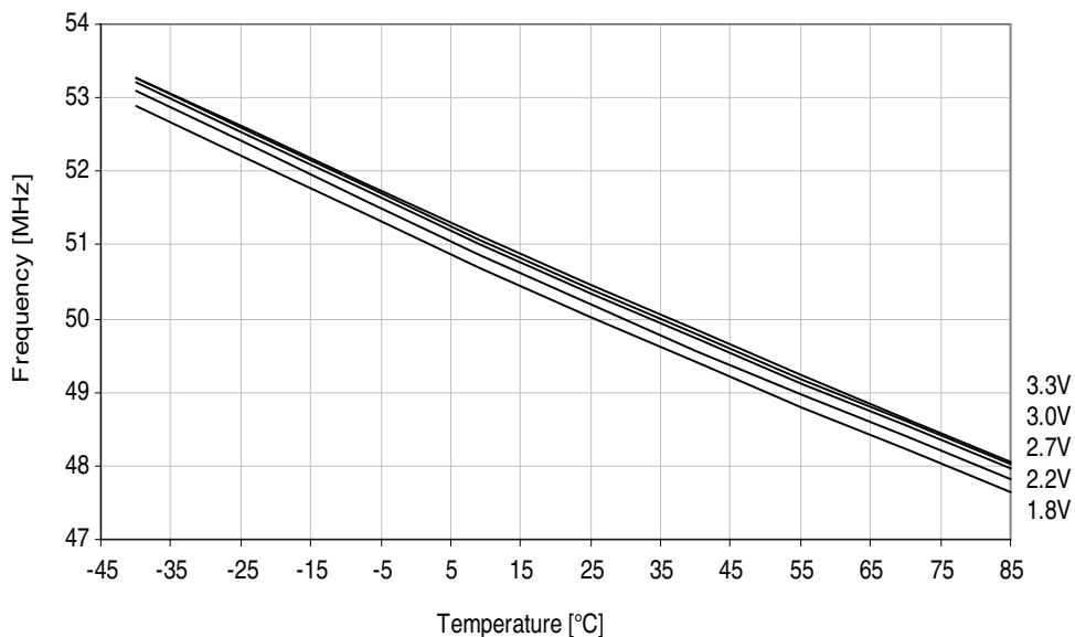
Figure 33-62. 48MHz internal oscillator frequency vs. temperature.
