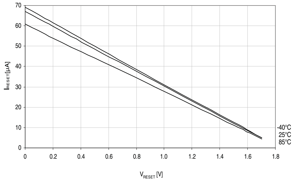
Figure 33-46. Reset pin pull-up resistor current vs. reset pin voltage.
