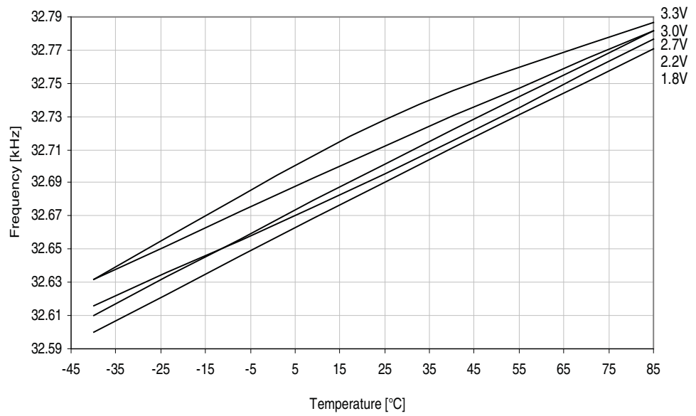
Figure 33-53. 32.768kHz internal oscillator frequency vs. temperature.
