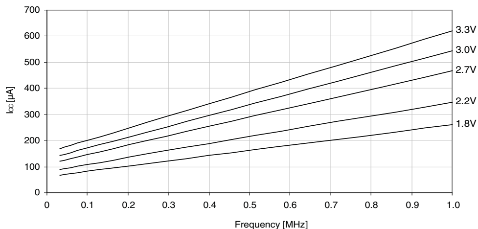
Figure 33-1. Active supply current vs. frequency.
