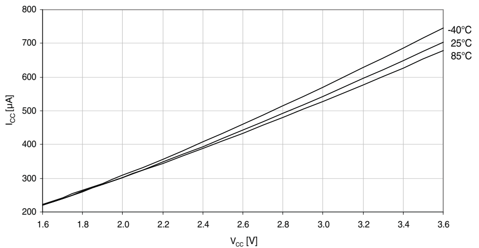
Figure 33-4. Active mode supply current vs. V_{CC} . f_{SYS} = 1\text{MHz} external clock.
