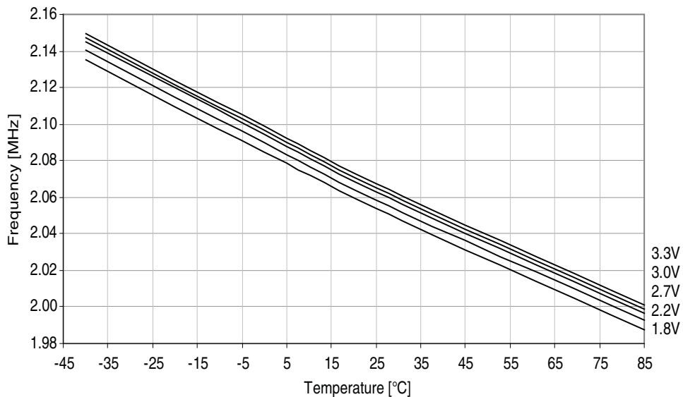
Figure 33-55. 2MHz internal oscillator frequency vs. temperature. DPLL disabled.
