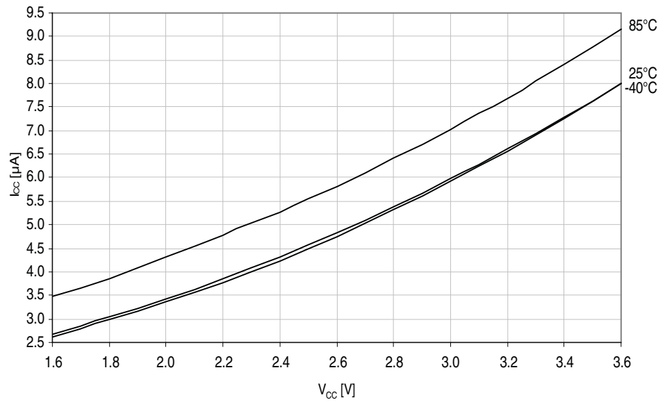
Figure 33-19. Standby supply current vs. V_{CC} .
