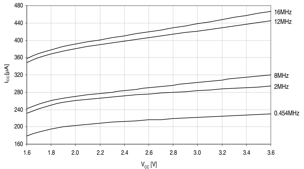
Figure 33-20. Standby supply current vs. V_{CC} .
