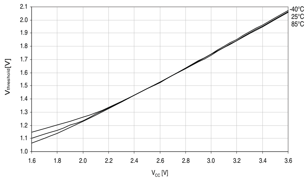
Figure 33-48. Reset pin input threshold voltage vs. V_{CC} .
