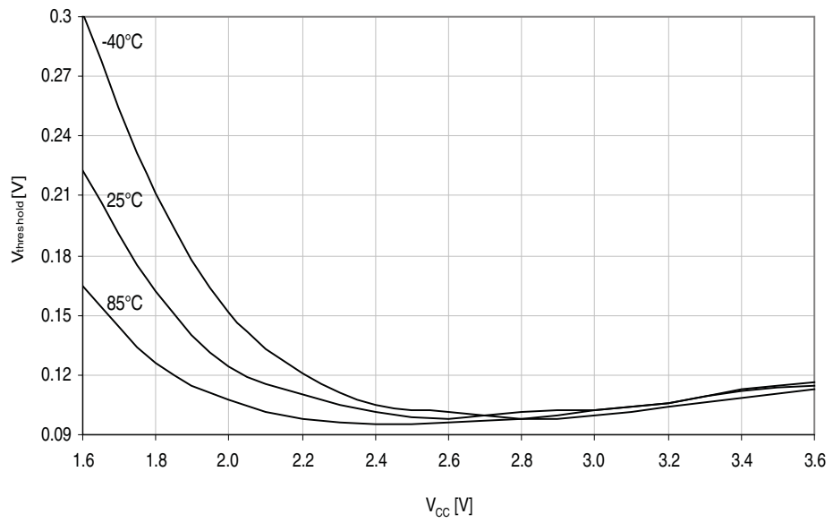
Figure 33-35. I/O pin input hysteresis vs. V_{CC} .
