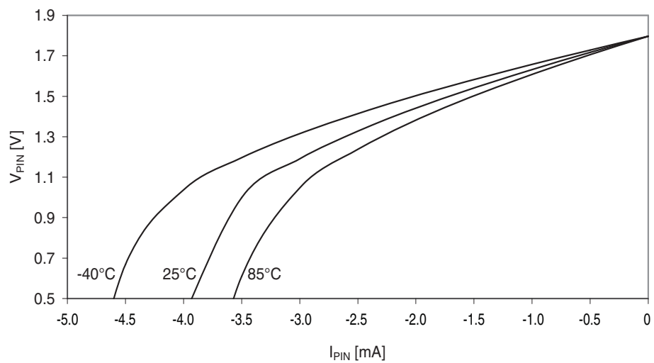
Figure 33-24. I/O pin output voltage vs. source current.
