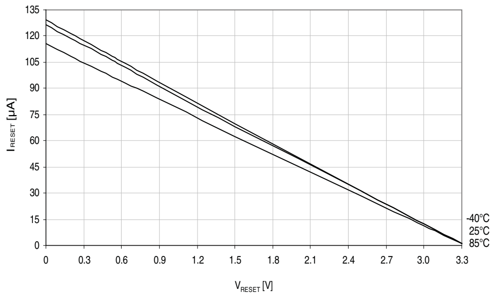
Figure 33-47. Reset pin pull-up resistor current vs. reset pin voltage.
