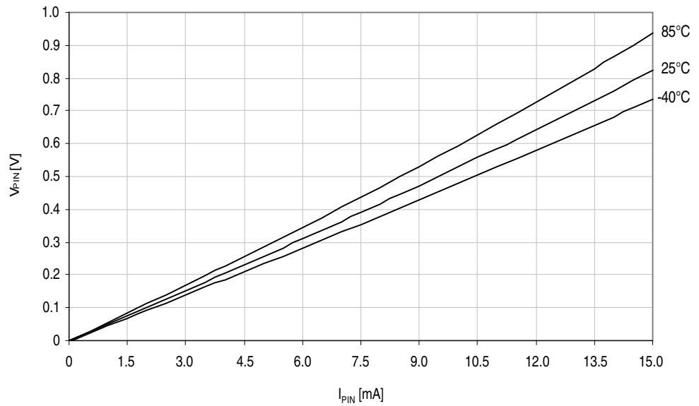
Figure 33-29. I/O pin output voltage vs. sink current.
