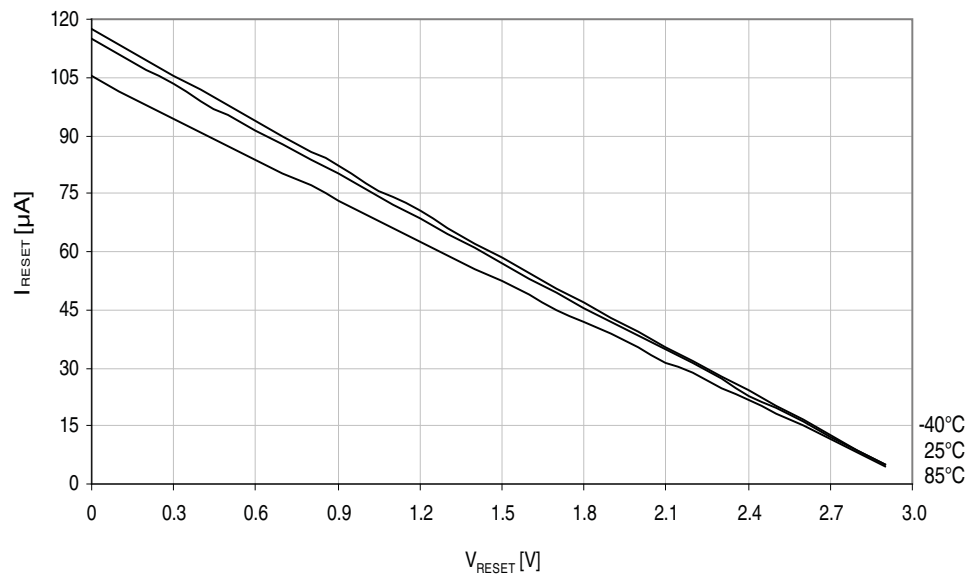
Figure 33-46. Reset pin pull-up resistor current vs. reset pin voltage.
