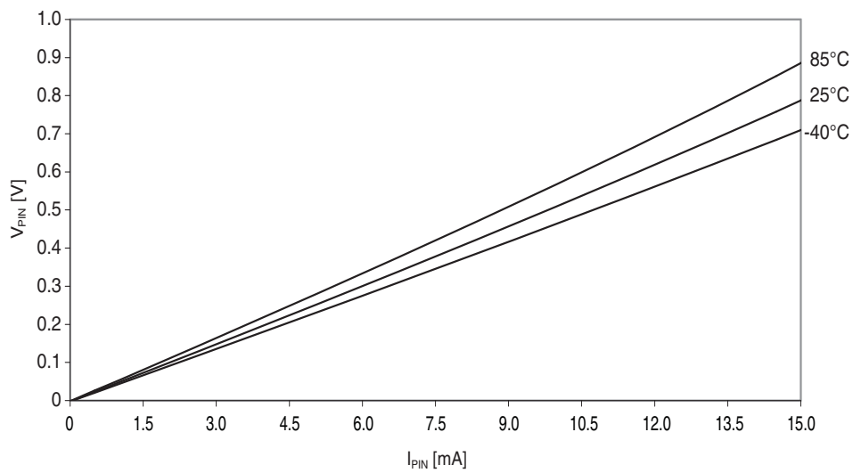
Figure 33-30. I/O pin output voltage vs. sink current.
