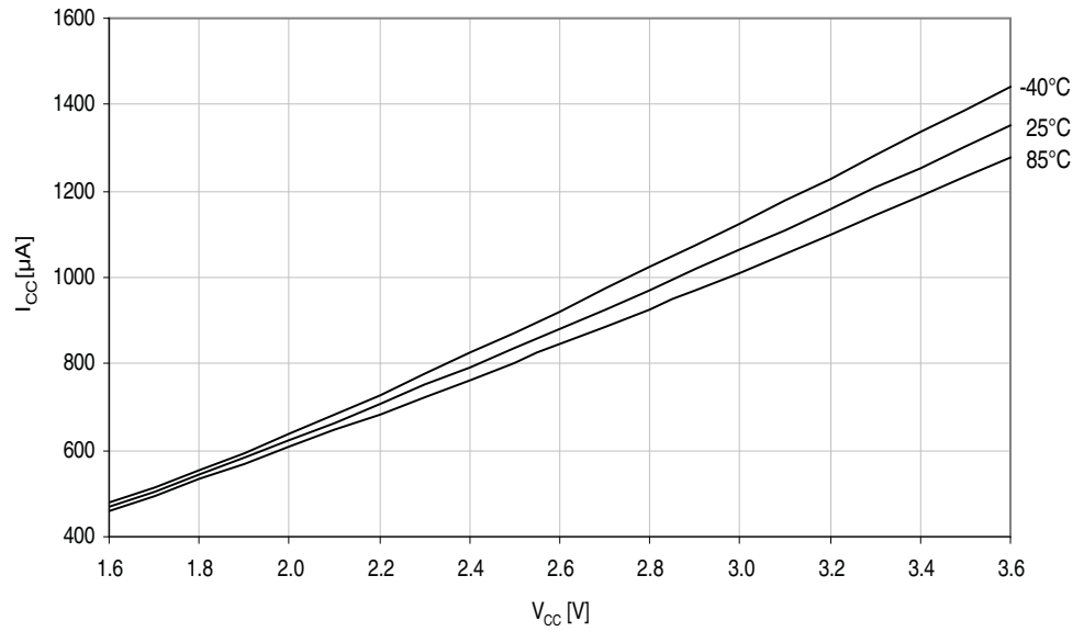
Figure 33-5. Active mode supply current vs. V_{CC} . f_{SYS} = 2MHz internal oscillator.
