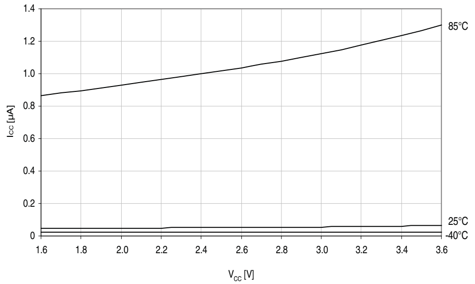
Figure 33-16. Power-down mode supply current vs. V_{CC} . All functions disabled.
