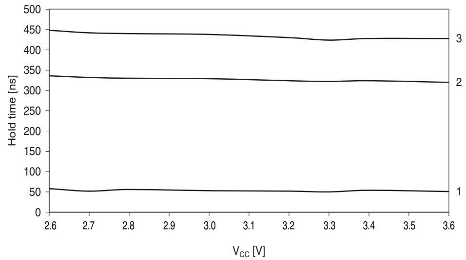
Figure 33-66. SDA hold time vs. supply voltage.
