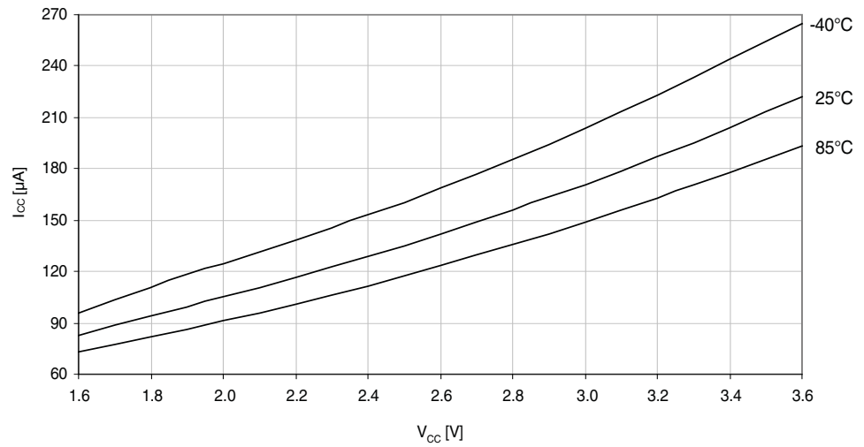
Figure 33-3. Active mode supply current vs. V_{CC} . f_{SYS} = 32.768\text{kHz} internal oscillator.
