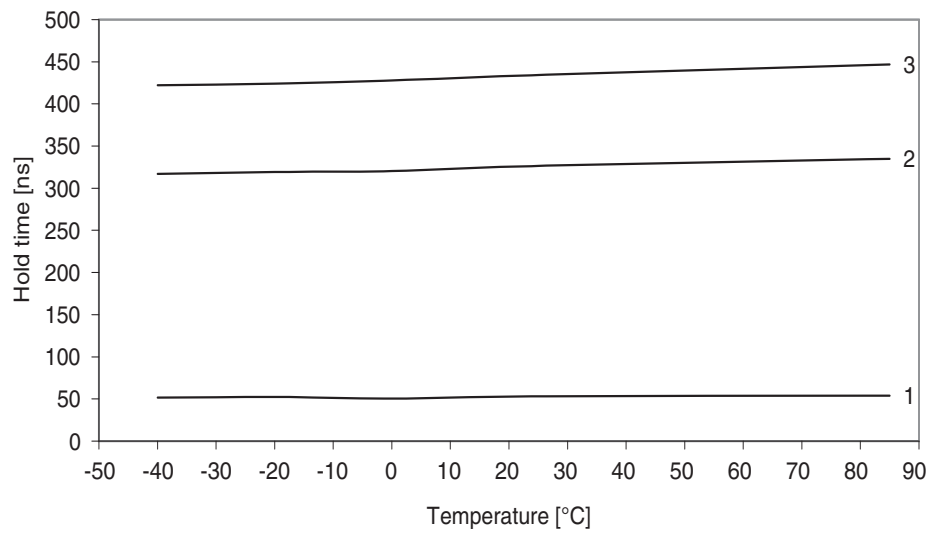
Figure 33-65. SDA hold time vs. temperature.
