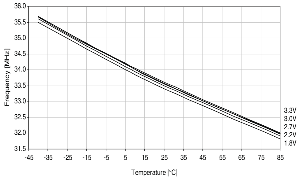
Figure 33-58. 32MHz internal oscillator frequency vs. temperature.
