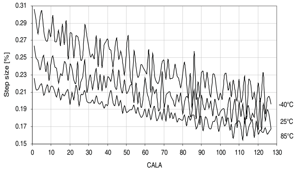
Figure 33-57. 2MHz internal oscillator CALA calibration step size.
