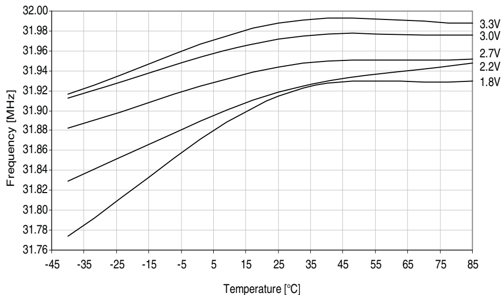
Figure 33-59. 32MHz internal oscillator frequency vs. temperature. DPLL enabled, from the 32.768kHz internal oscillator.
