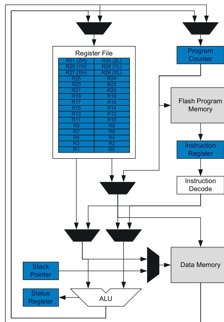
Figure 6-1. Block diagram of the AVR CPU architecture.
