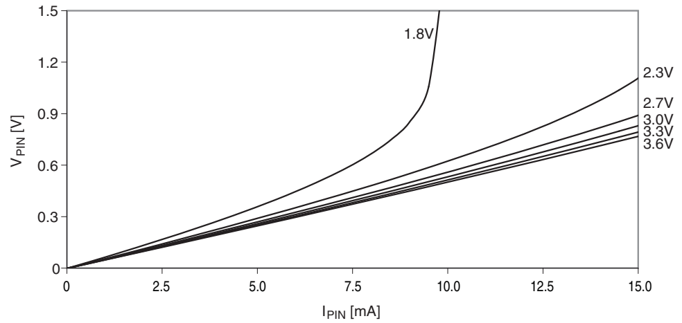
Figure 33-31. I/O pin output voltage vs. sink current.
