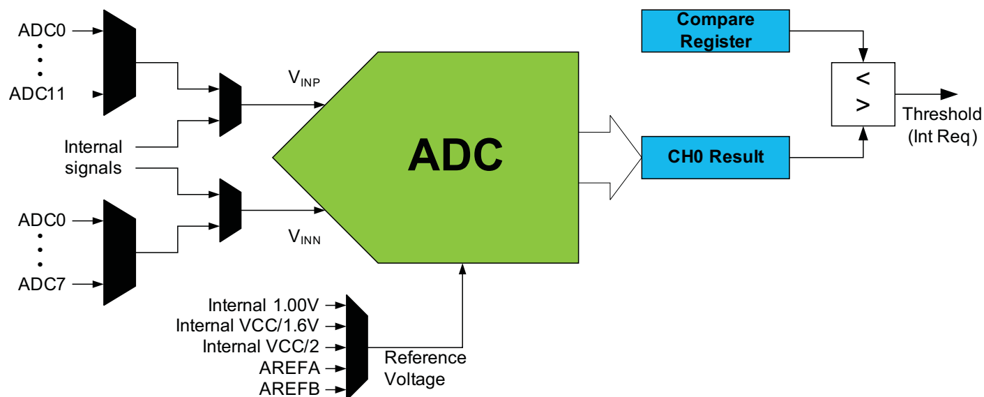
Figure 25-1. ADC overview.
