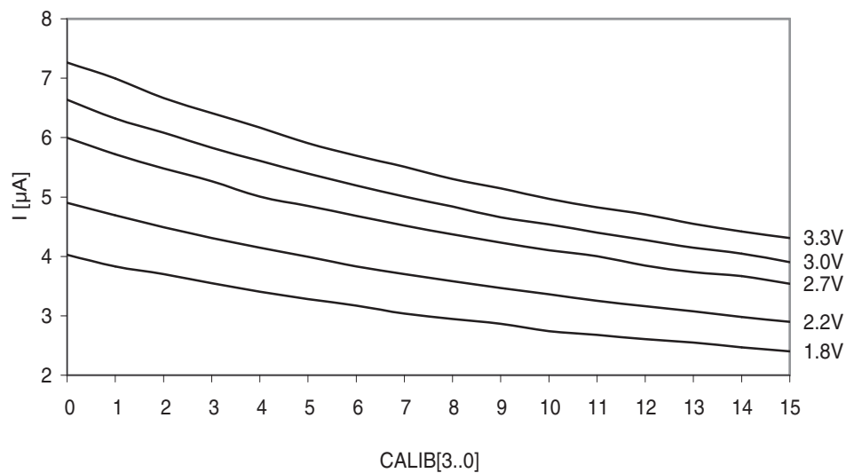
Figure 33-38. Analog comparator current source vs. calibration value.
