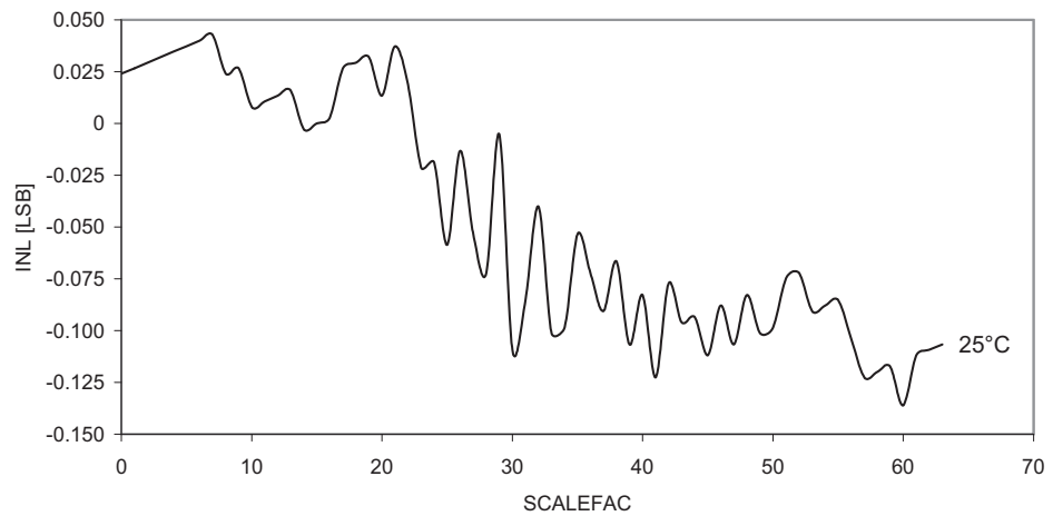
Figure 33-40. Voltage scaler INL vs. SCALEFAC.
