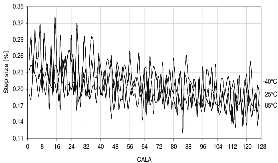
Figure 33-64. 48MHz internal oscillator CALA calibration step size.
