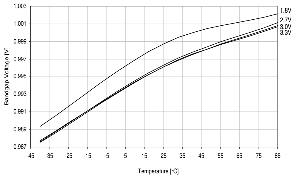
Figure 33-41. ADC internal 1.0V reference vs. temperature.
