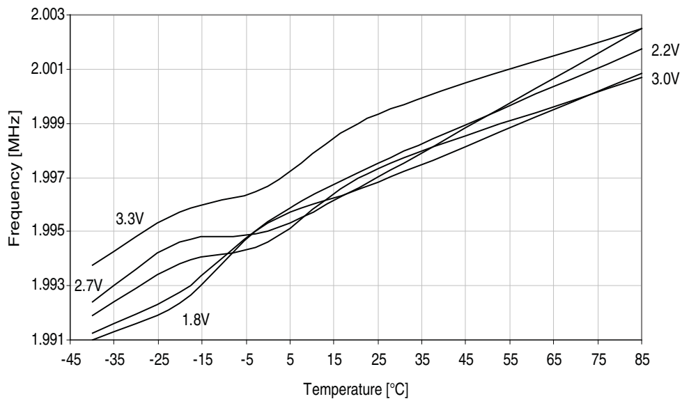
Figure 33-56. 2MHz internal oscillator frequency vs. temperature. DPLL enabled, from the 32.768kHz internal oscillator.
