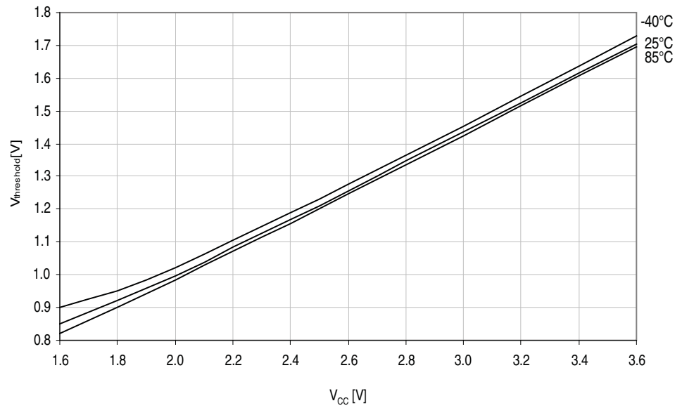
Figure 33-33. I/O pin input threshold voltage vs. V_{CC} .
