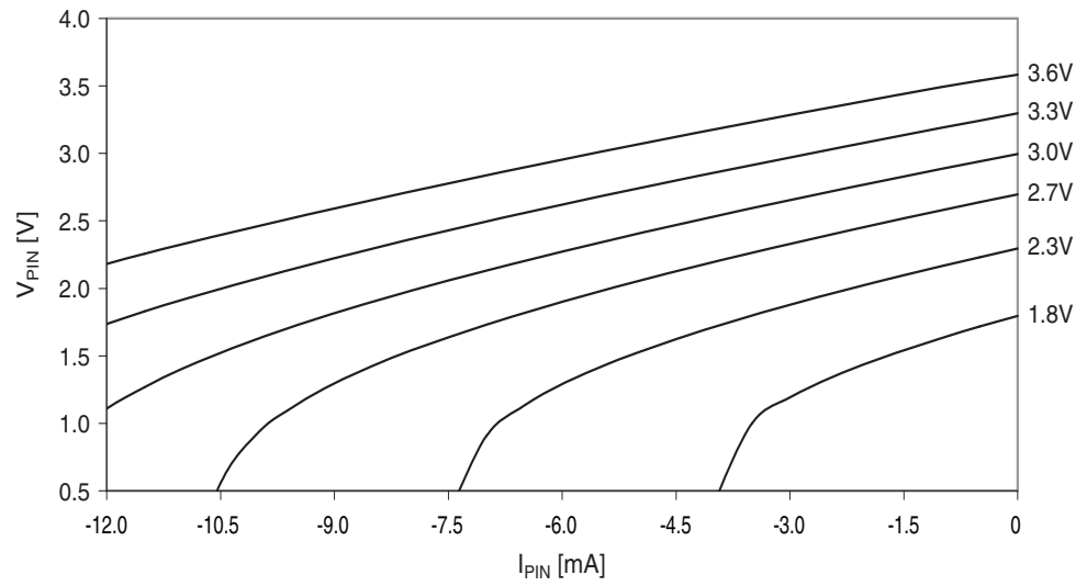
Figure 33-27. I/O pin output voltage vs. source current.
