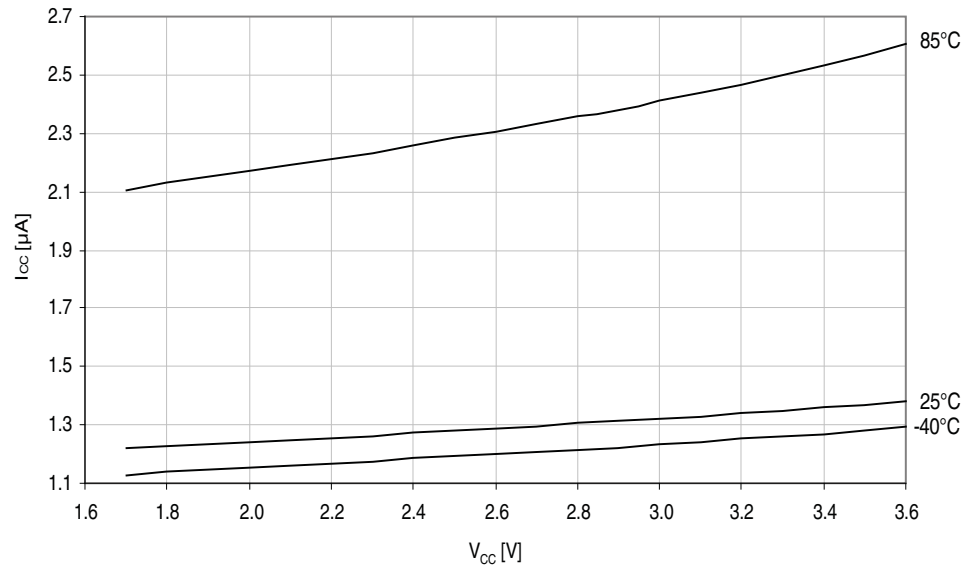
Figure 33-17. Power-down mode supply current vs. V_{CC} . Watchdog and sampled BOD enabled.
