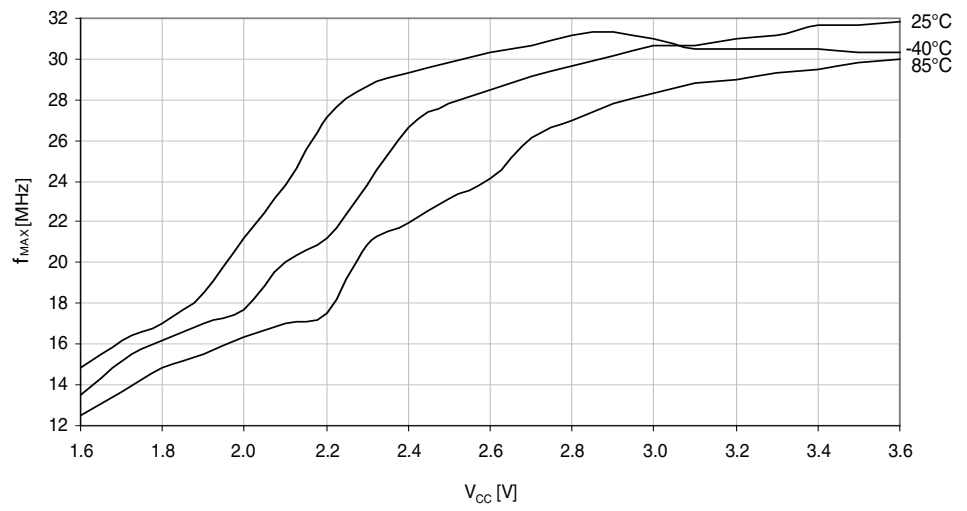
Figure 33-67. Maximum PDI frequency vs. V_{CC} .
