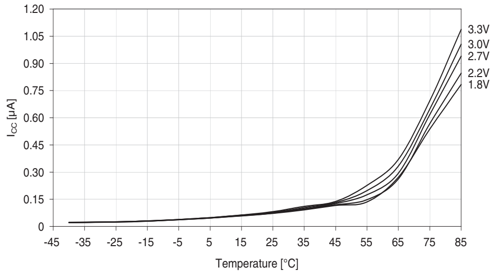
Figure 33-15. Power-down mode supply current vs. temperature. All functions disabled.
