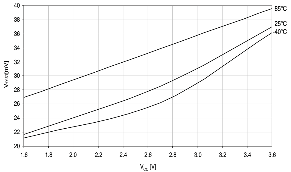
Figure 33-37. Analog comparator hysteresis vs. V_{CC} .
