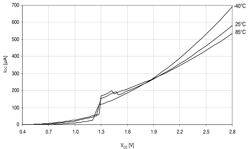
Figure 33-50. Power-on reset current consumption vs. V_{CC} . BOD level = 3.0V, enabled in continuous mode.
