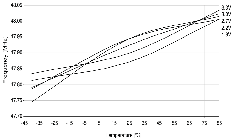
Figure 33-63. 48MHz internal oscillator frequency vs. temperature.
