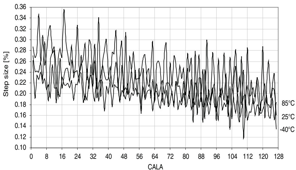
Figure 33-60. 32MHz internal oscillator CALA calibration step size. V CC = 3.0V.
