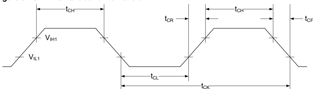
Figure 32-3. External clock drive waveform.
