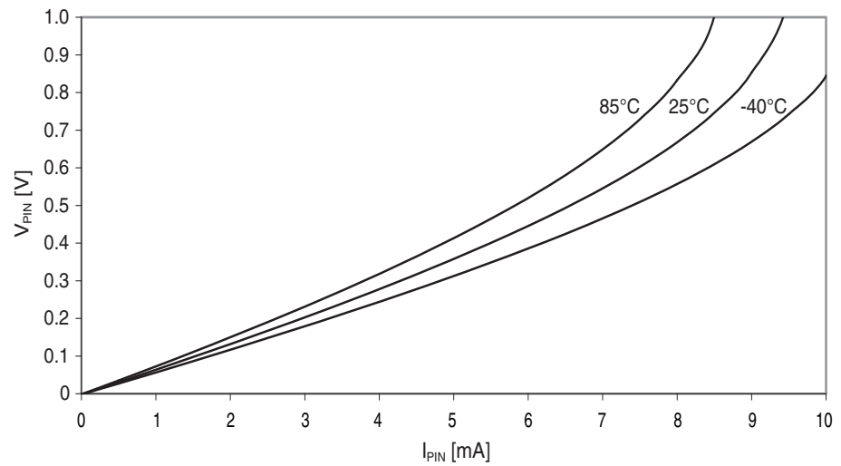
Figure 33-28. I/O pin output voltage vs. sink current.
