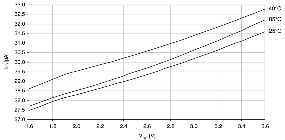
Figure 33-10. Idle mode supply current vs. V_{CC} .
