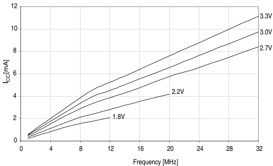
Figure 33-2. Active supply current vs. frequency.
