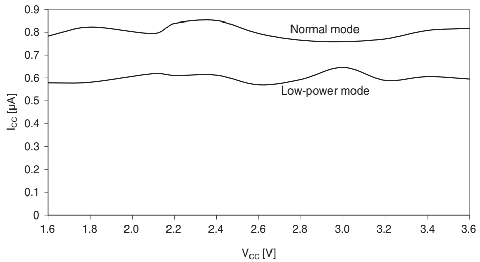
Figure 33-18. Power-save mode supply current vs. V_{CC} . Real Time Counter enabled and running from 1.024kHz output of 32.768kHz TOSC.
