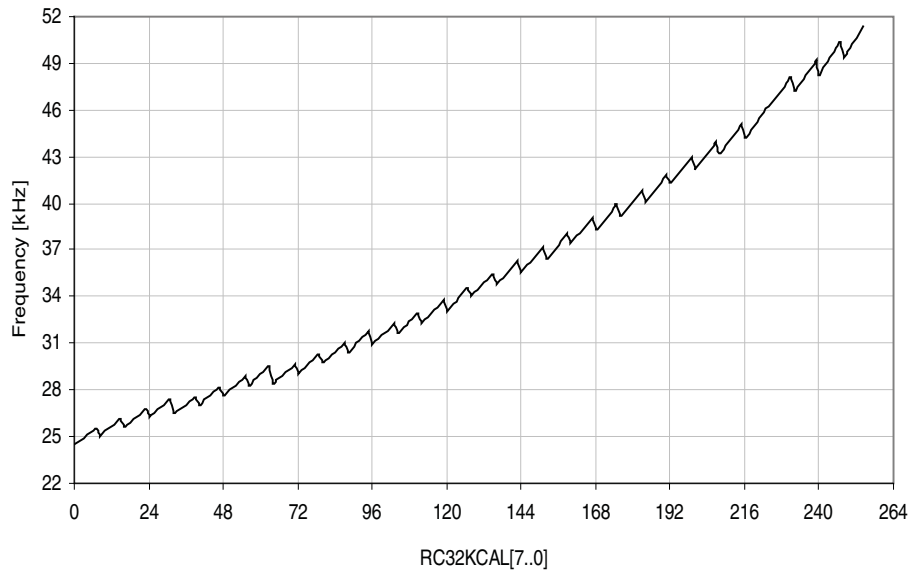
Figure 33-54. 32.768kHz internal oscillator frequency vs. calibration value.
