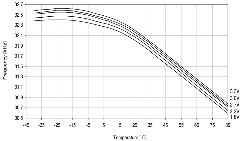
Figure 33-52. Ultra Low-Power internal oscillator frequency vs. temperature.
