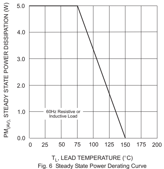
Fig. 6 Steady State Power Derating Curve
