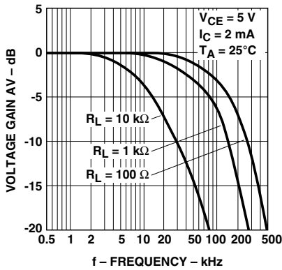
Figure 10. Frequency response.
