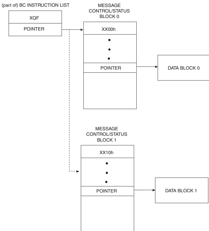
FIGURE 4. EXECUTE and FLIP (XQF) OPERATION
