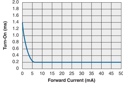
Typical Turn-On vs. LED Forward Current ( I_L=1\text{A}_{\text{DC}} )
