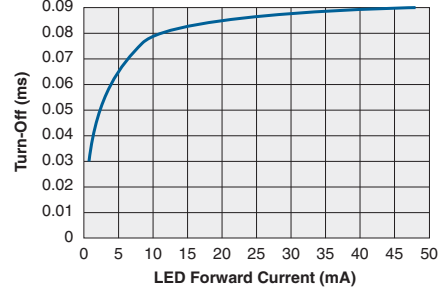
Typical Turn-Off vs. LED Forward Current ( I_L=1\text{A}_{\text{DC}} )
