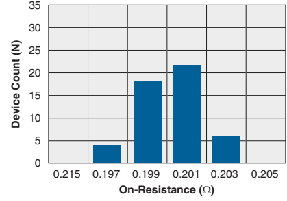
Typical On-Resistance Distribution (N=50, I_F=10\text{mA} , I_L=1\text{A}_{\text{DC}} , T_A=25^\circ\text{C} )
