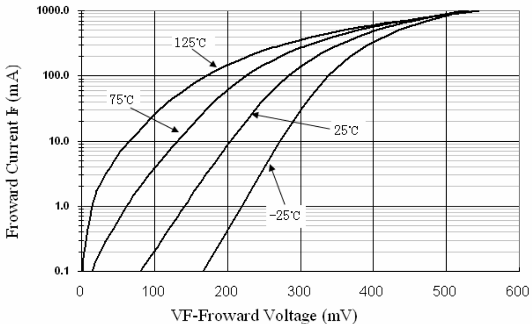
Forward Voltage vs Ambient Temperature
