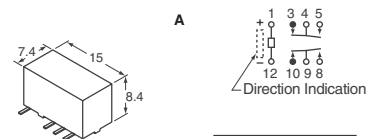
Fig. 21 — TXD Series NEW!
