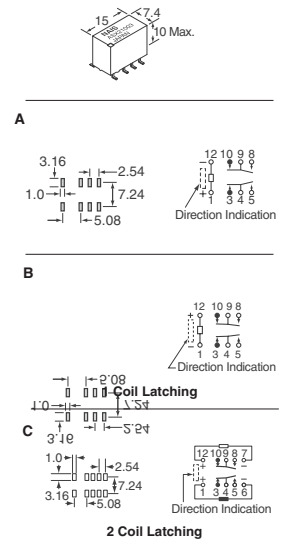
Fig. 13 — TK Series
