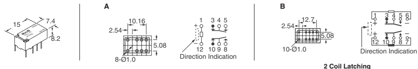
Fig. 18 — TX and TXS Series - PCB
