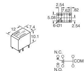
Fig. 10 — HY Series
