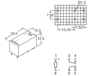
Fig. 4 — DE Series
