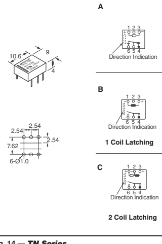
Fig. 14 — TN Series
