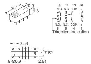
Fig. 9 — HX Series
