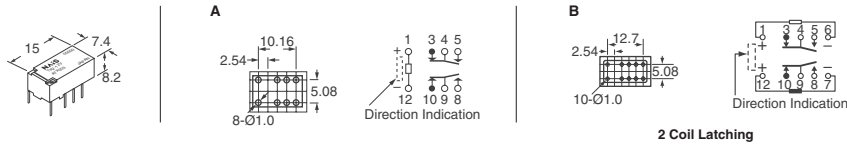
Fig. 18 — TX and TXS Series - PCB
