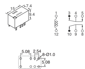
Fig. 10 — HY Series
