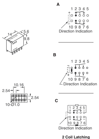
Fig. 14 — TN Series
