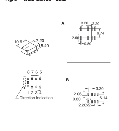
Fig. 2 — AGQ Series - SMD
