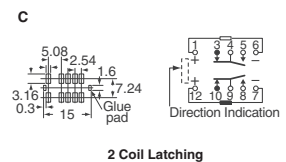
Fig. 21 — TXD Series NEW!
