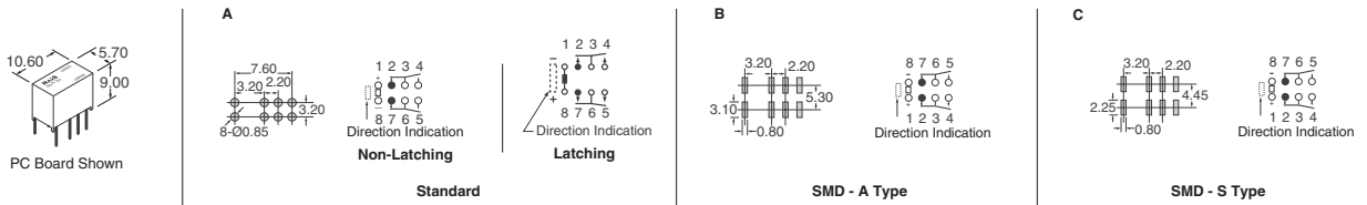
Fig. 4 — DE Series
