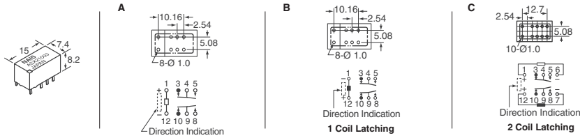
Fig. 11 — ASX Series
