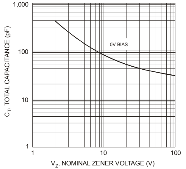
Fig. 2 Typical Capacitance
