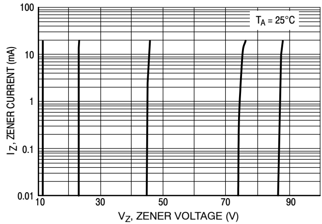
Figure 8. Zener Voltage versus Zener Current ( V_Z 12 V to 91 V)
