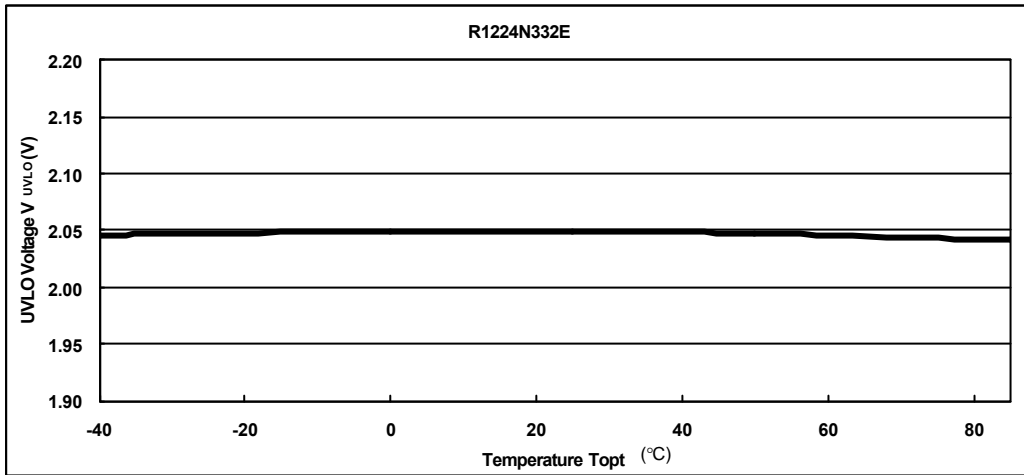
13) UVLO Voltage vs. Temperature
