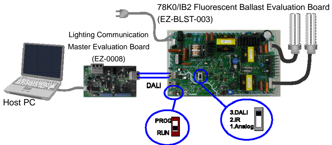
Figure 7. DALI Protocol control
