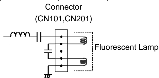
Figure 3. Pin assignment of Lamp connector(CN101, CN201)
