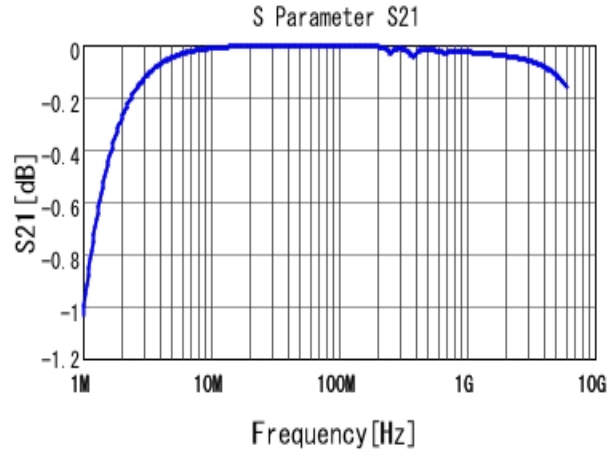
■ GRM1885C1H302JA01 S21 DCOV, 25degC
