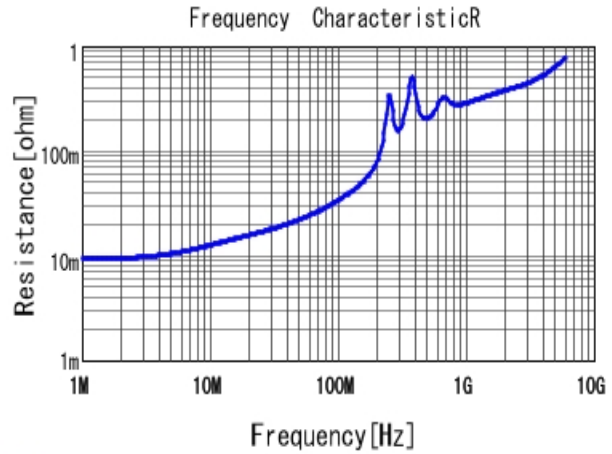
■ GRM1885C1H302JA01 R DCOV, 25degC
