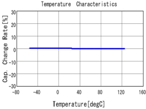
■ GRM1885C1H302JA01 C-Temp. capchange, DCOV, AC1Vrms
