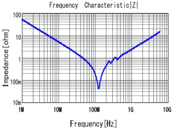
■ GRM1885C1H302JA01 |Z| DCOV, 25degC
