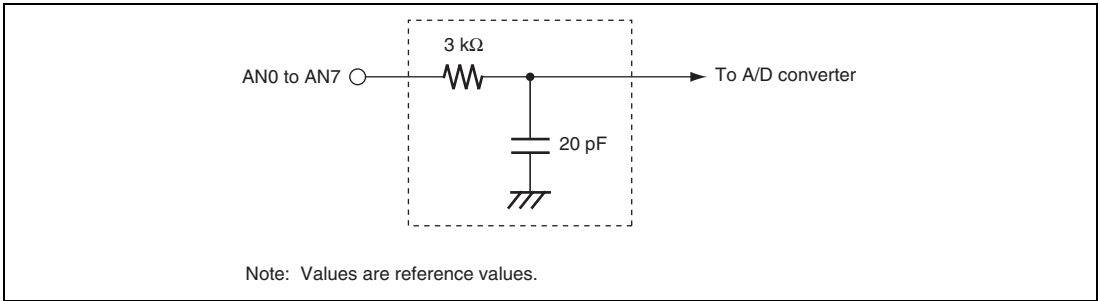
Figure 20.9 Analog Input Pin Equivalent Circuit
