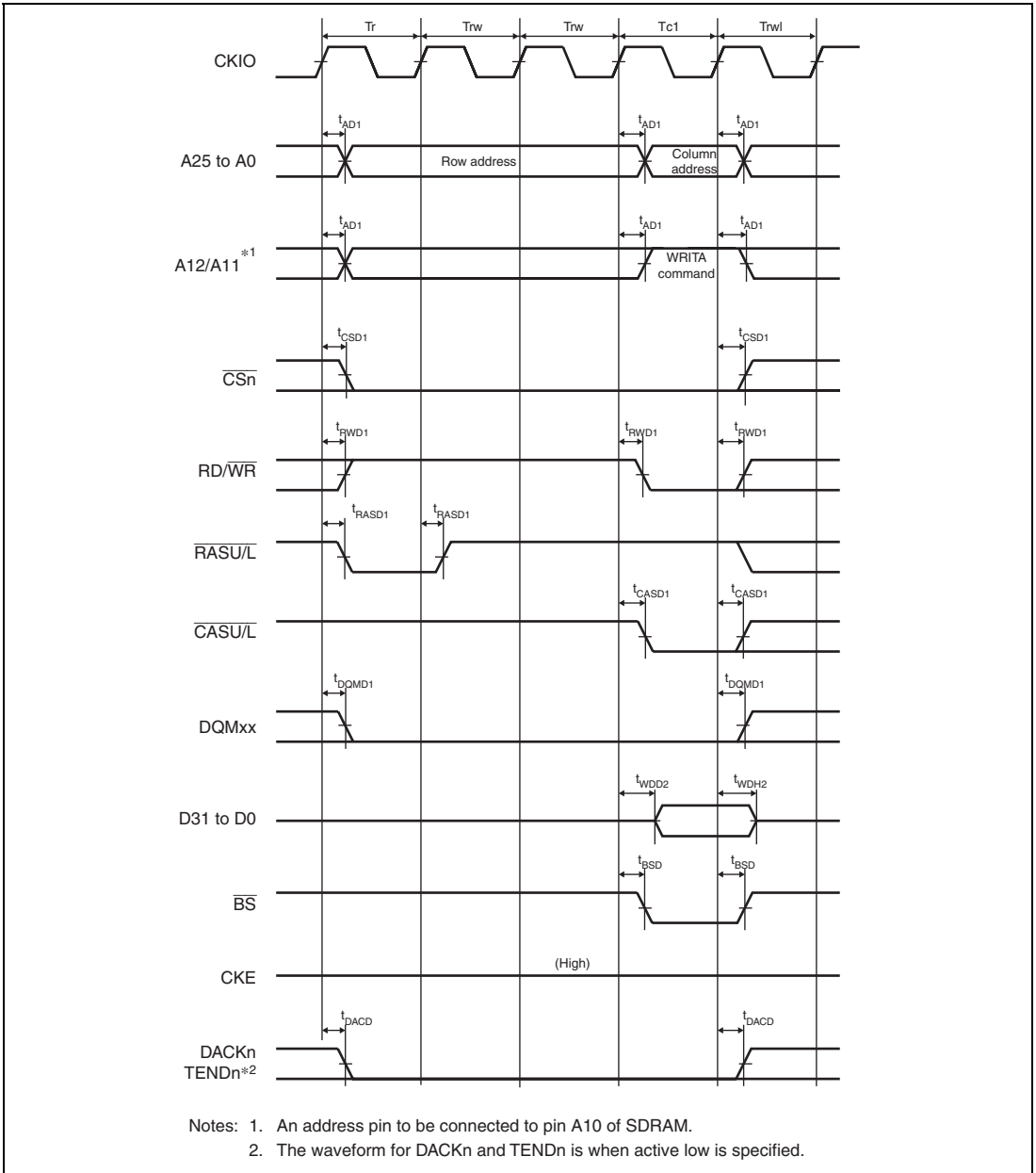
Figure 31.27 Synchronous DRAM Single Write Bus Cycle (Auto Precharge, WTRCD = 2 Cycles, TRWL = 1 Cycle)
