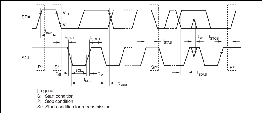
Figure 31.57 IIC3 Input/Output Timing
