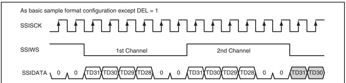
Figure 18.16 Transmitting and Receiving in the Order of Serial Data and Padding Bits; without Delay
