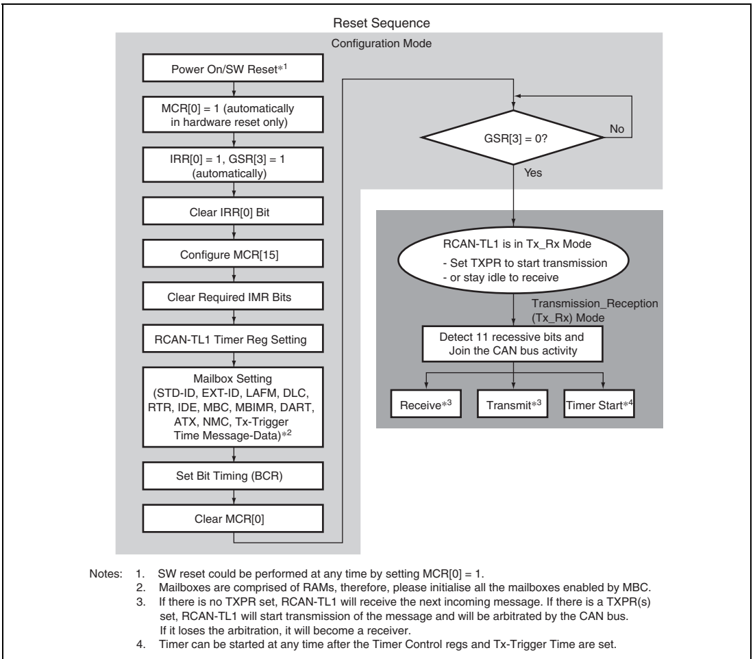
Figure 19.14 Reset Sequence
