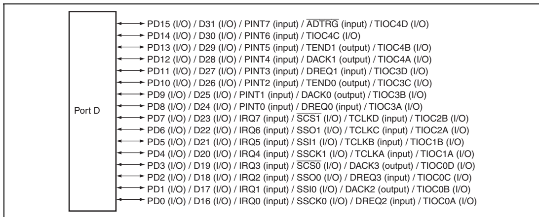
Figure 26.4 Port D
