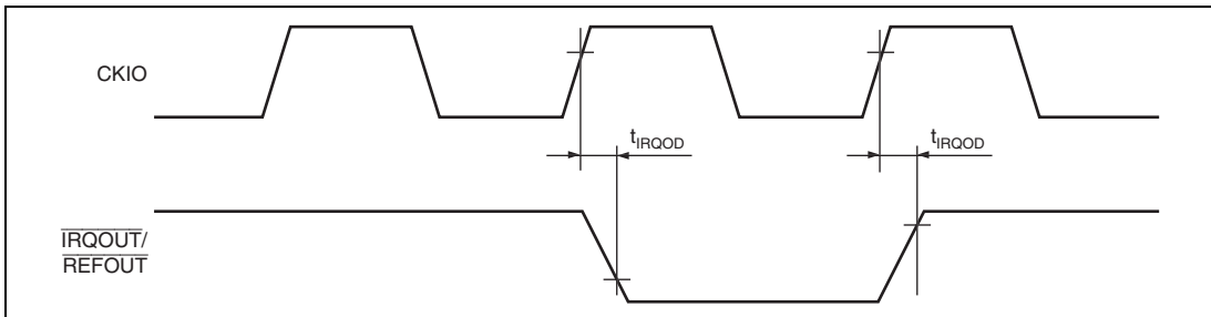
Figure 31.11 Interrupt Signal Output Timing
