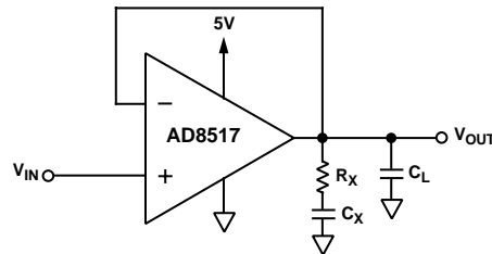
Figure 24. Snubber Network Compensation for Capacitive Loads
