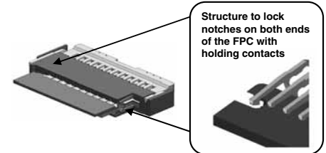
Applicable FPC shape
