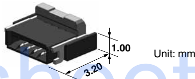
4 pin contacts (Y5B: minimum)
