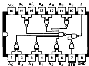
C12 DM8160N 6-bit comparator
