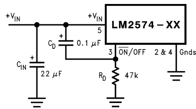
FIGURE 15. Delayed Startup
