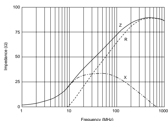
BLM31AF700SN1
