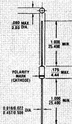
FIGURE 1 All dimensions in \frac{\text{INCH}}{\text{m.m.}}
