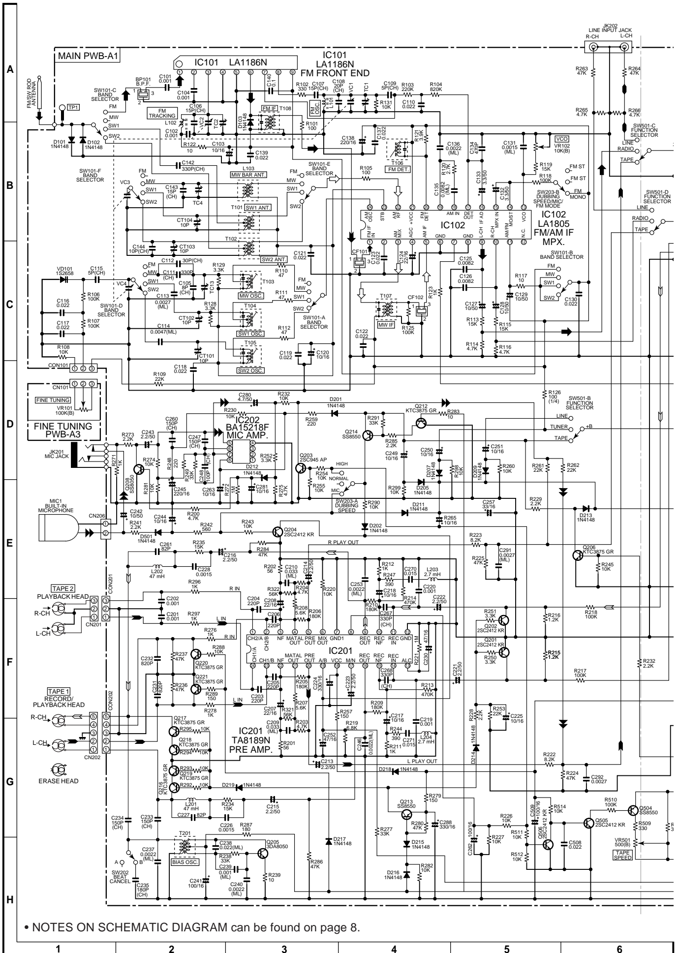
Figure 10 SCHEMATIC DIAGRAM (1/2)
