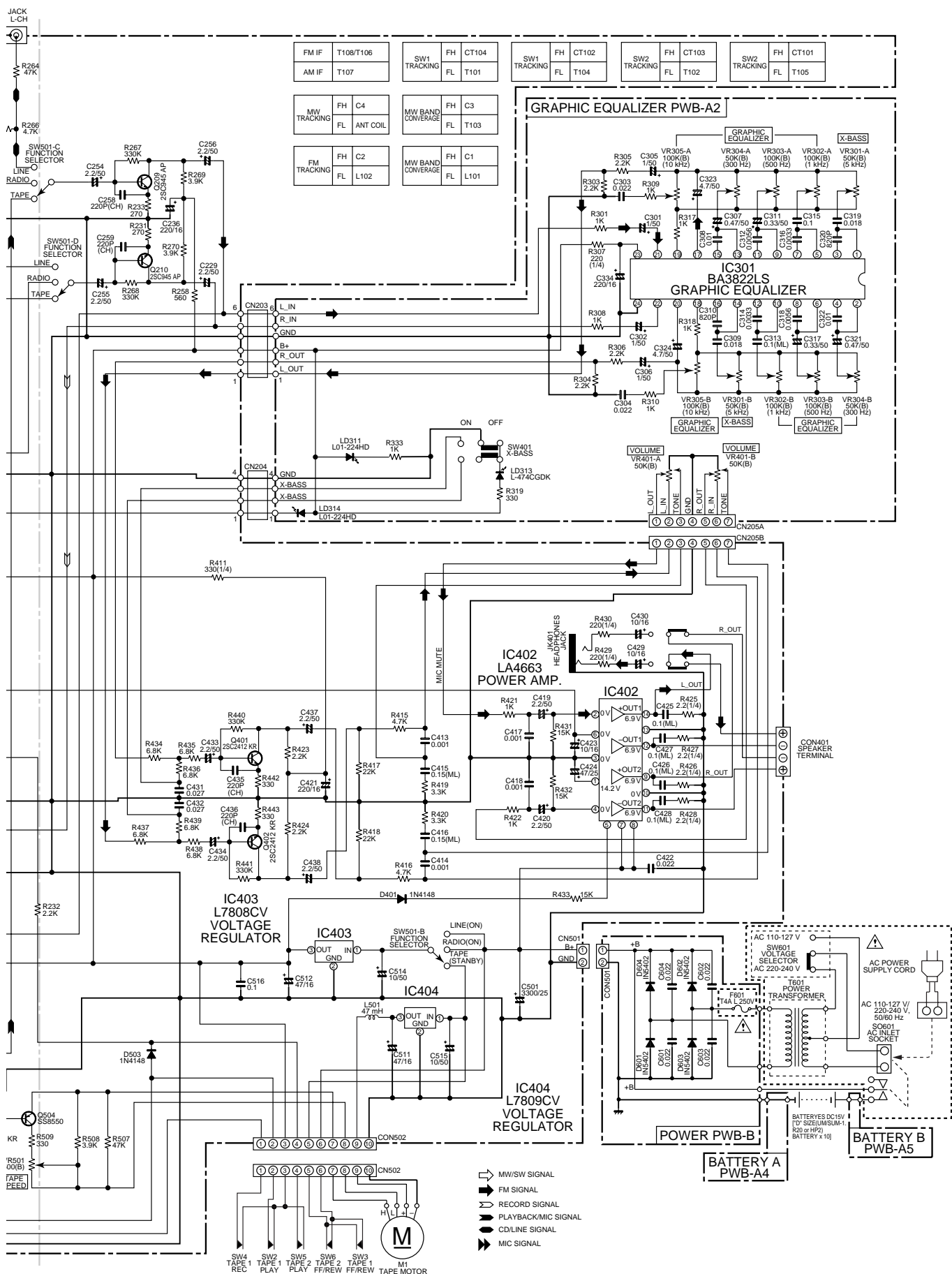
Figure 11 SCHEMATIC DIAGRAM (2/2)
