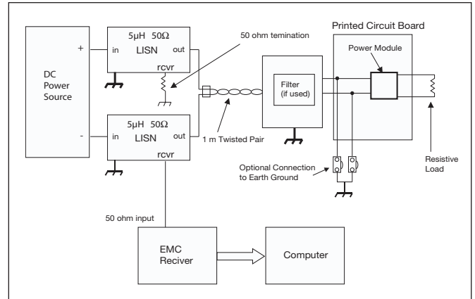
Test set-up.
