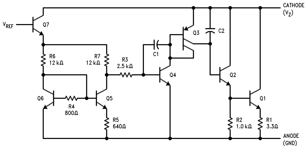
Figure 11. Equivalent Circuit
