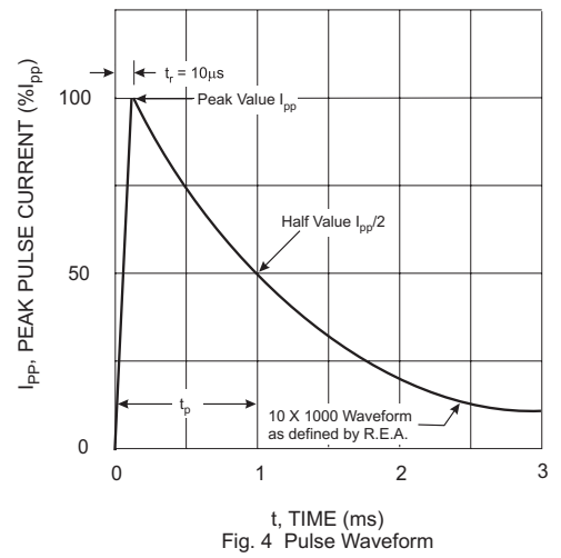
Fig. 4 Pulse Waveform
