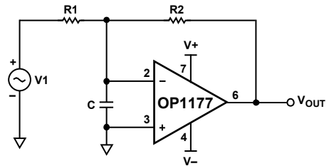
Figure 61. EMI Reduction
