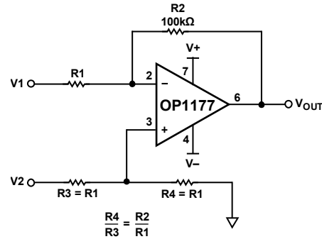
Figure 63. Difference Amplifier
