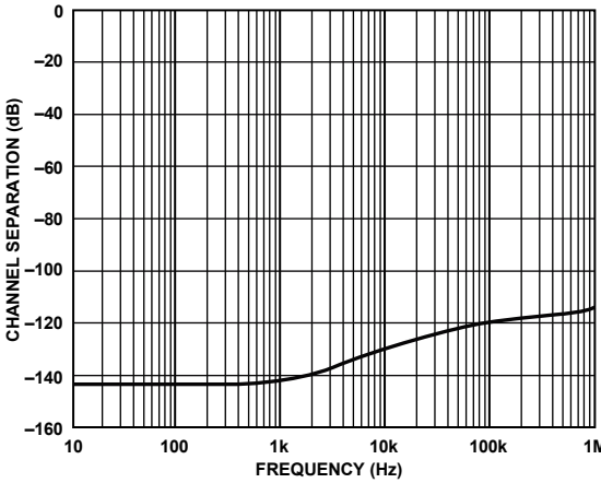
Figure 50. Channel Separation vs. Frequency
