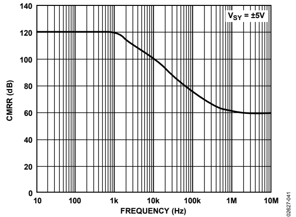
Figure 41. CMRR vs. Frequency
