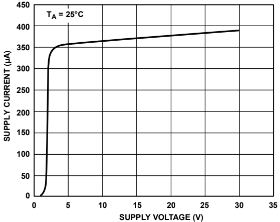
Figure 49. Supply Current vs. Supply Voltage
