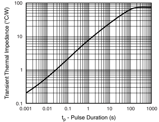
Figure 12. Typical Transient Thermal Impedance
