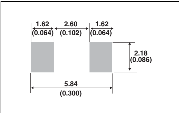
Figure 13. Footprint dimensions in mm (inches)
