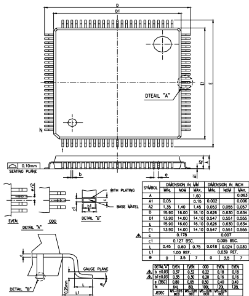
128-Pin LQFP Package
