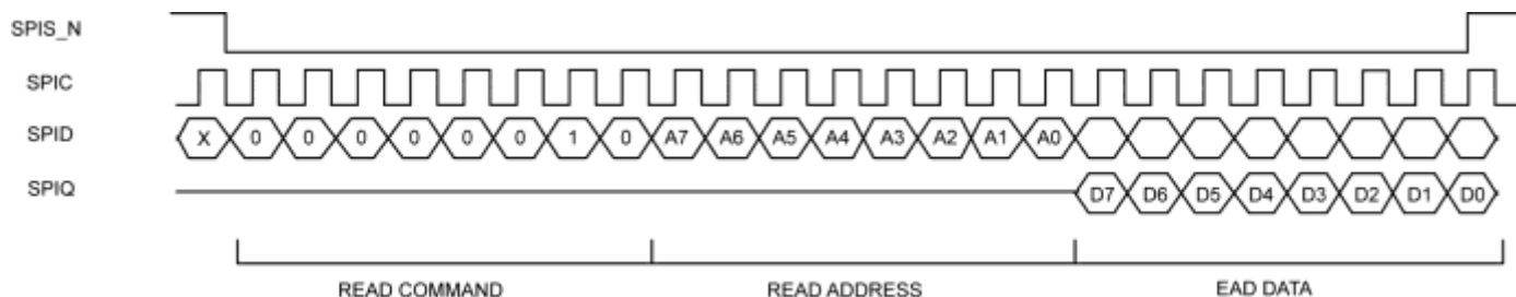
Figure 16. SPI Read Data Cycle
