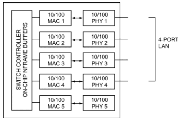
Figure 3. Standalone Switch
